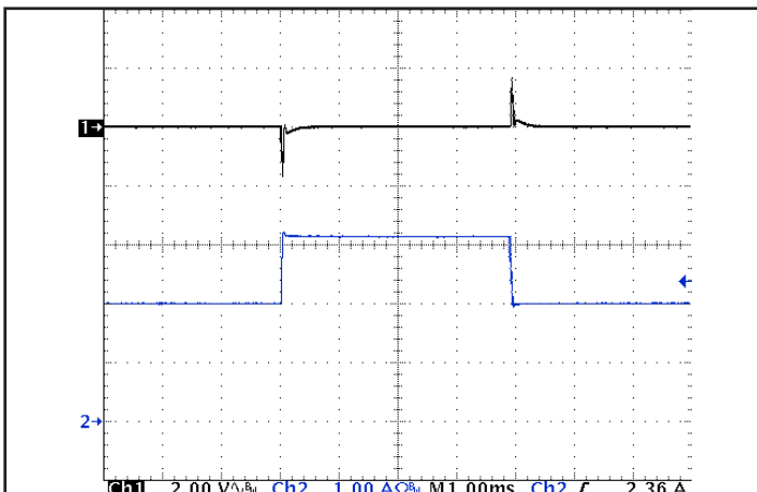
Figure 5: Output voltage response to step-change in load current (66% - 100% - 66% of I out (max); di/dt = 0.1 A/μs). Load cap: 15 μF tantalum cap and 1 μF ceramic cap. Ch 1: V out (2 V/div), Ch 2: I out (1 A/div).
