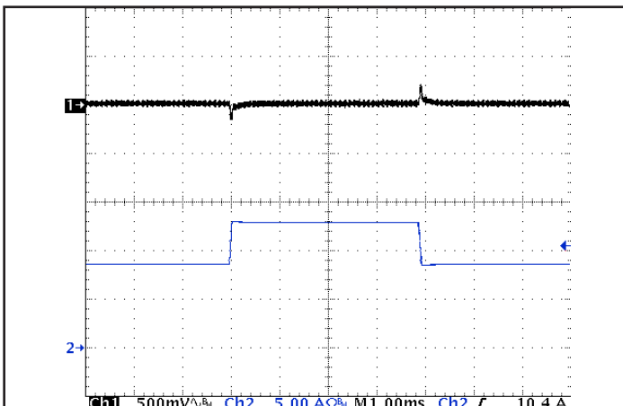
Figure 5: Output voltage response to step-change in load current (66% -100% -66% of I out (max); dI/dt = 0.1 A/μs). Load cap: 15 μF tantalum cap and 1 μF ceramic cap. Ch 1: V out (500 mV/div), Ch 2: I out (5 A/div).
