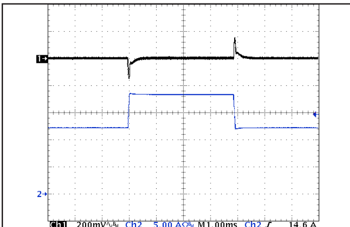
Figure 5: Output voltage response to step-change in load current (66% -100% -66% of I_{out(max)} ; dI/dt = 0.1 A/\mu s ). Load cap: 15 \mu F tantalum cap and 1 \mu F ceramic cap. Ch 1: V_{out} (200 mV/div), Ch 2: I_{out} (5 A/div).
