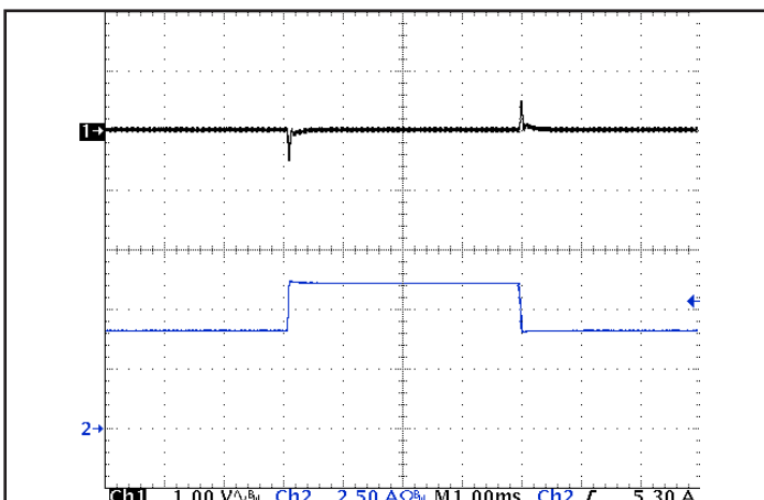
Figure 5: Output voltage response to step-change in load current (66% -100% -66% of I out (max); dI/dt = 0.1 A/μs). Load cap: 15 μF tantalum cap and 1 μF ceramic cap. Ch 1: V out (1 V/div), Ch 2: I out (2.5 A/div).
