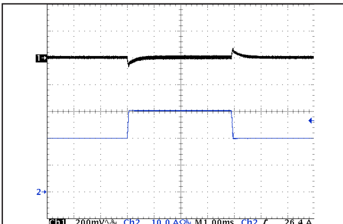
Figure 5: Output voltage response to step-change in load current (66% - 100% - 66% of I out (max); dl/dt = 0.1 A/μs). Load cap: 15 μF tantalum cap and 1 μF ceramic cap. Ch 1: V out (200 mV/div), Ch 2: I out (10 A/div).
