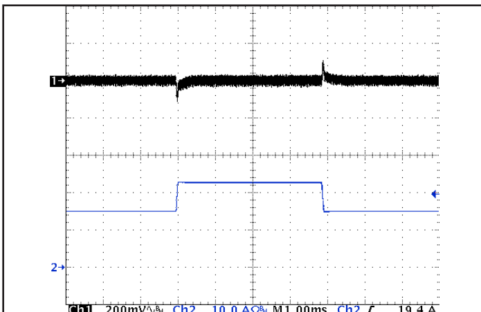
Figure 5: Output voltage response to step-change in load current (66% -100% -66% of I out (max); dI/dt = 0.1 A/μs). Load cap: 15 μF tantalum cap and 1 μF ceramic cap. Ch 1: V out (200 mV/div), Ch 2: I out (10 A/div).
