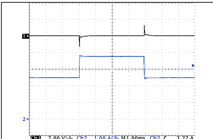
Figure 5: Output voltage response to step-change in load current (66% -100% -66% of I out (max); dI/dt = 0.1 A/μs). Load cap: 15 μF tantalum cap and 1 μF ceramic cap. Ch 1: V out (2 V/div), Ch 2: I out (1 A/div).
