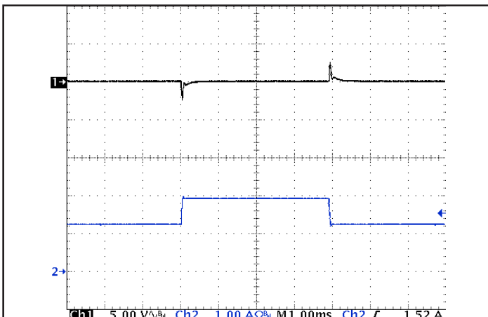
Figure 5: Output voltage response to step-change in load current (66% -100% -66% of I out (max); dI/dt = 0.1 A/μs). Load cap: 15 μF tantalum cap and 1 μF ceramic cap. Ch 1: V out (5 V/div), Ch 2: I out (1 A/div).
