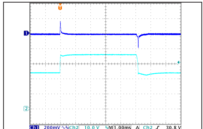
Figure 6: Output voltage response to step-change in input voltage (nominal to maximum), at full load current. Load cap: 100 \mu F , electrolytic output capacitance. Ch 1: V_{out} , Ch 2: V_{in} .
